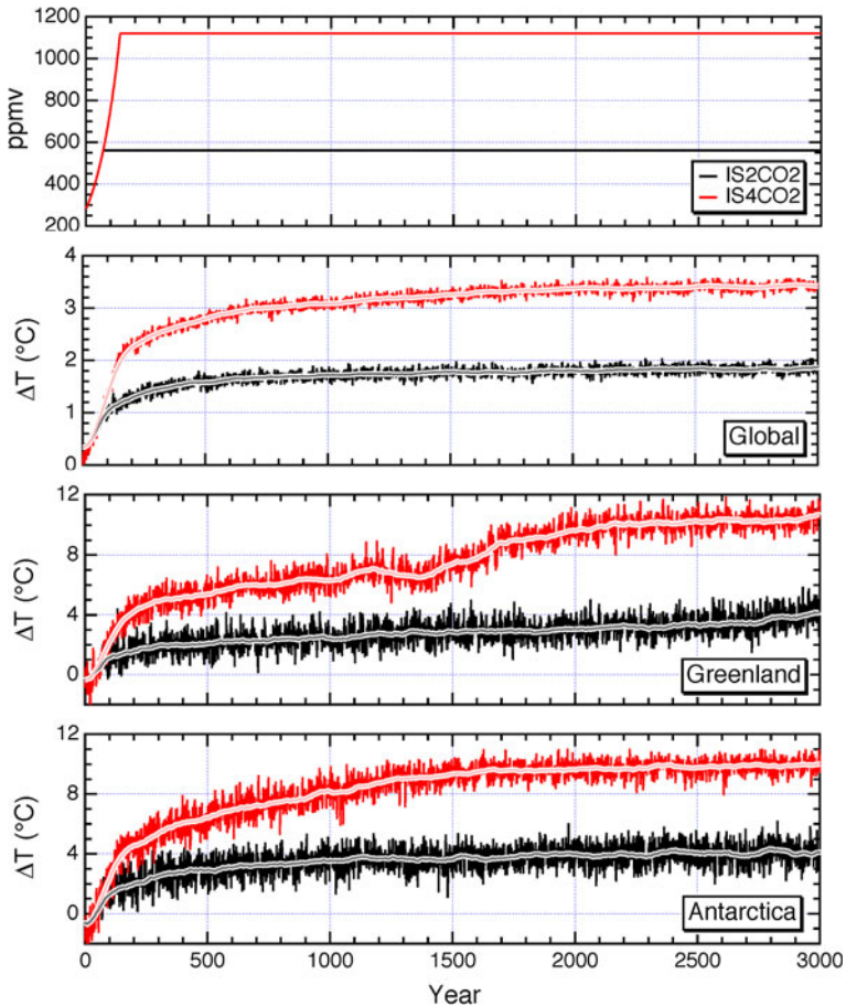
Fig. 3 The experiments employed two CO 2 forcing scenarios, respectively doubling (IS2CO 2 , black lines) and quadrupling (IS4CO 2 , red lines) the pre-industrial concentration of 280 ppmv. Shown are the corresponding time evolution of the CO 2 concentration, global mean annual temperature, and mean annual temperature over Greenland and Antarctica. The lower three panels display the full yearly variability of mean temperature around the 100 years running mean
